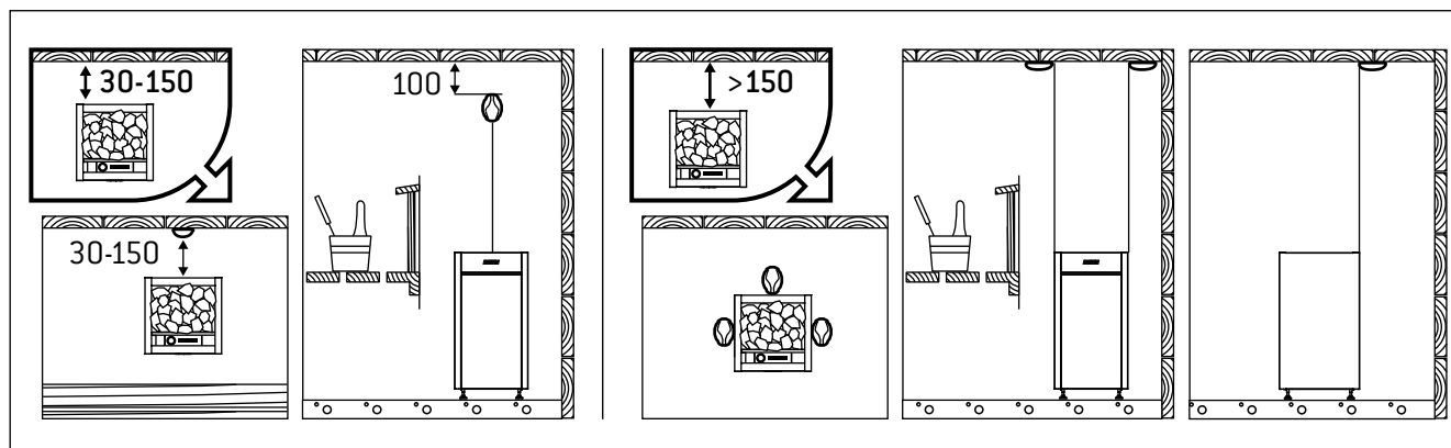
Figure 7. Installing the temperature sensor (all dimensions in millimeters) Abbildung 7. Installation der Temperaturfühler (alle Abmessungen in Millimetern)
